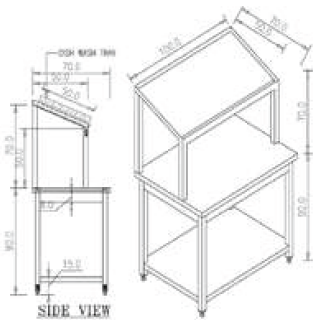
DISH LANDING TABLE
