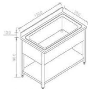
LARGE BOWL SINK
