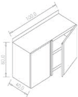
WALL CABINET
